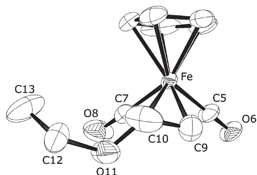
Fig. 2 ORTEP drawing (50% probability ellipsoids) of the non-hydrogen atoms of (\text{C}_5\text{H}_5)\text{Fe}(\text{CO})_2(\text{H}_2\text{C}=\text{CHOEt})^+ , showing selective atom labeling. The view angle is chosen to allow comparison to Fig. 1 and to emphasize their similarity. This has the consequence of falsely diminishing the real difference of the angle Fe–C α –C β .
