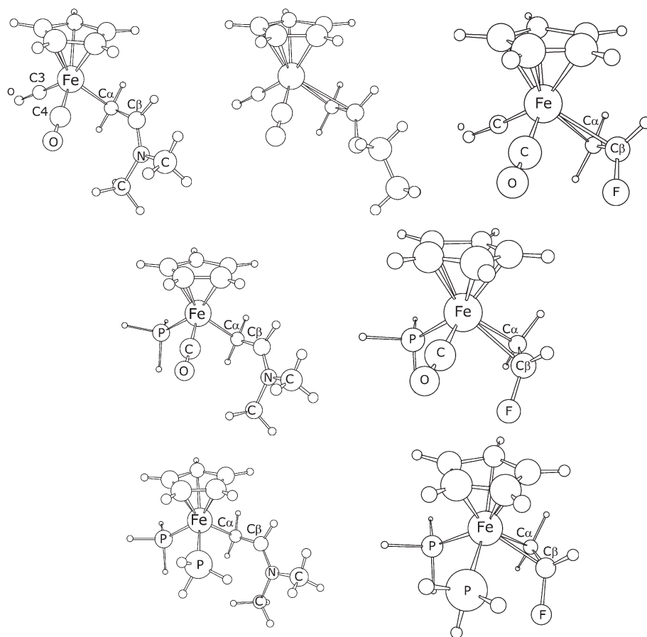
Fig. 3 DFT geometry-optimized structures (all are cations) of [CpFe(CO) n (PH 3 ) 2-n (H 2 C=CHD 0 )] + .
